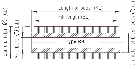
Wheel brush - standard version
