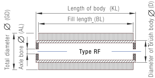
Wheel brush with inserted flange
